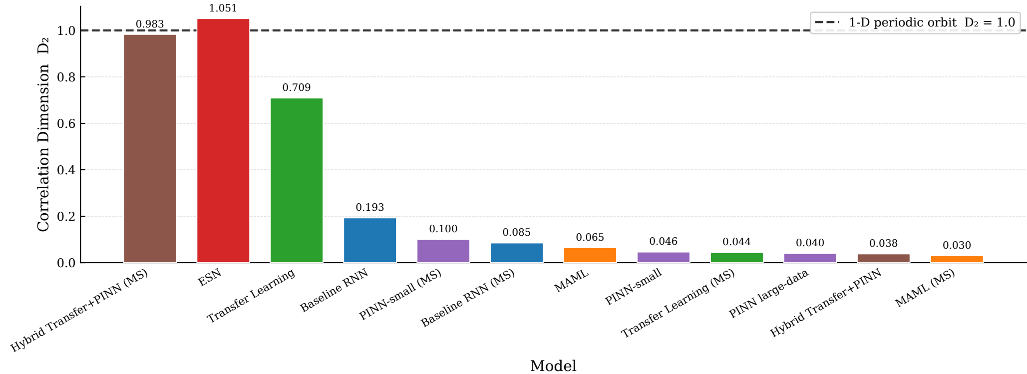
Duffing — Correlation Dimension D_2 Closer to reference line = better attractor reconstruction
